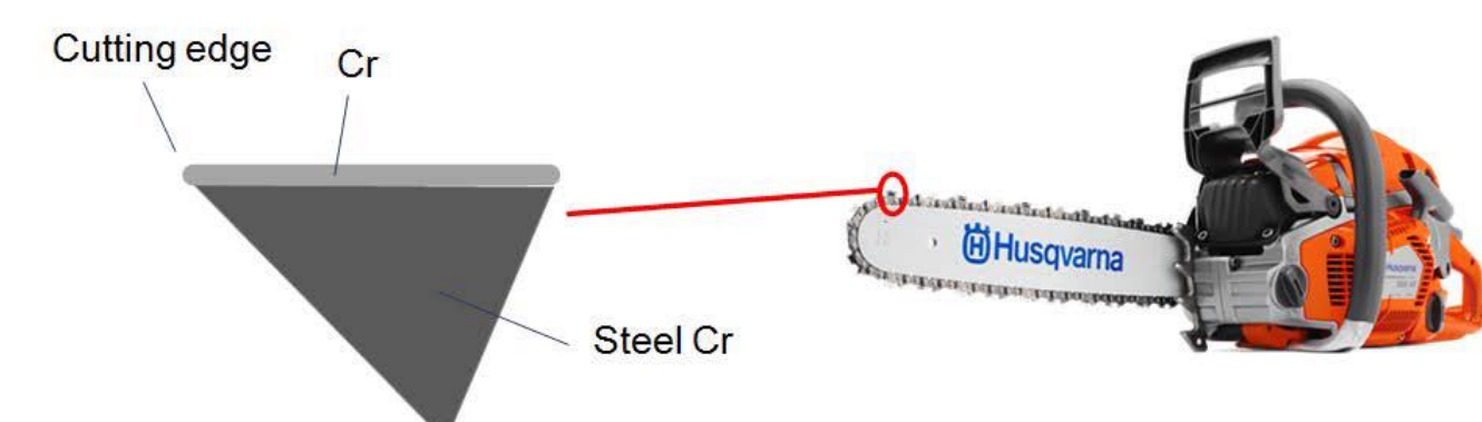
Cross-section of a cutting edge with Cr coating on a cutting link
