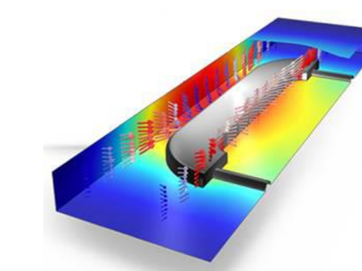
Current flow in electroplating of irregular shapes
